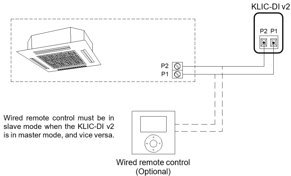
Figure 2. Connecting KLIC-DI v2 to the P1/P2 bus.
