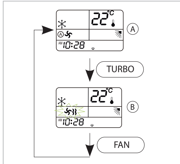
Abb. 18: Taste "Turbo"
